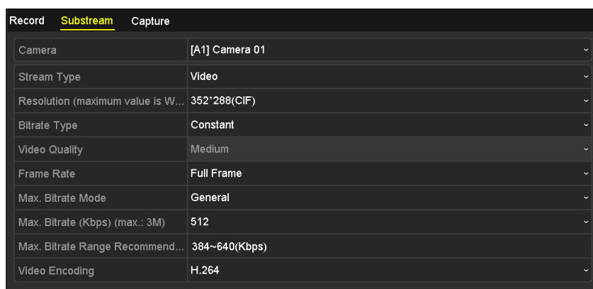
Figure 5-6 Sub-Stream Encoding
