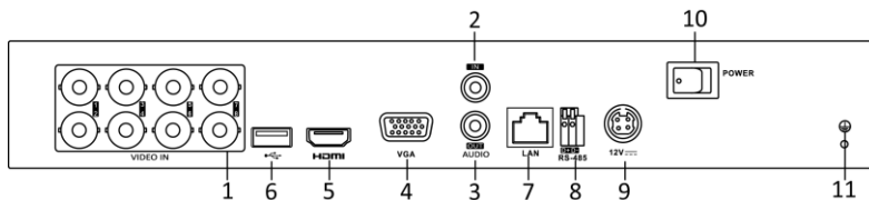
Figure 1-13 Rear Panel of DS-7200HGHI-E1/E2
