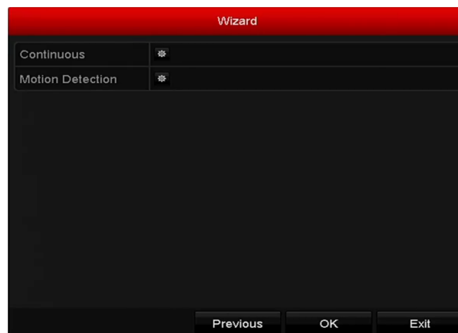
Figure 2-16 Record Settings
